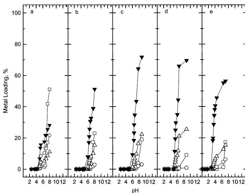
Figure 2. Percent metal loadings versus equilibrium pH of the aqueous phase for competitive solvent extraction of alkaline earth metal ions into chloroform by di-ionizable calix[4]arene-1,2-crown-5 ligands: (a) 6 , (b) 8 , (c) 9 , (d) 10 , and (e) 11 (□ = Mg 2+ ; ○ = Ca 2+ ; △ = Sr 2+ ; ▼ = Ba 2+ ). 12
